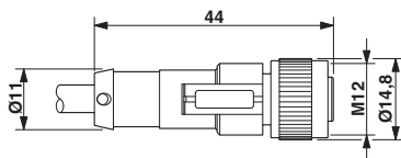
M12 x 1 female connector, straight
